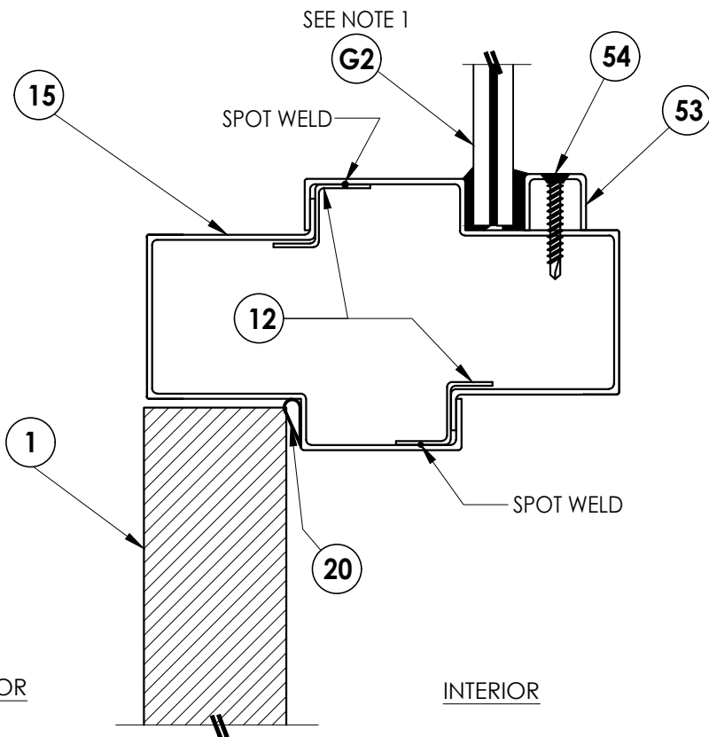
4 5 VERTICAL CROSS SECTION
