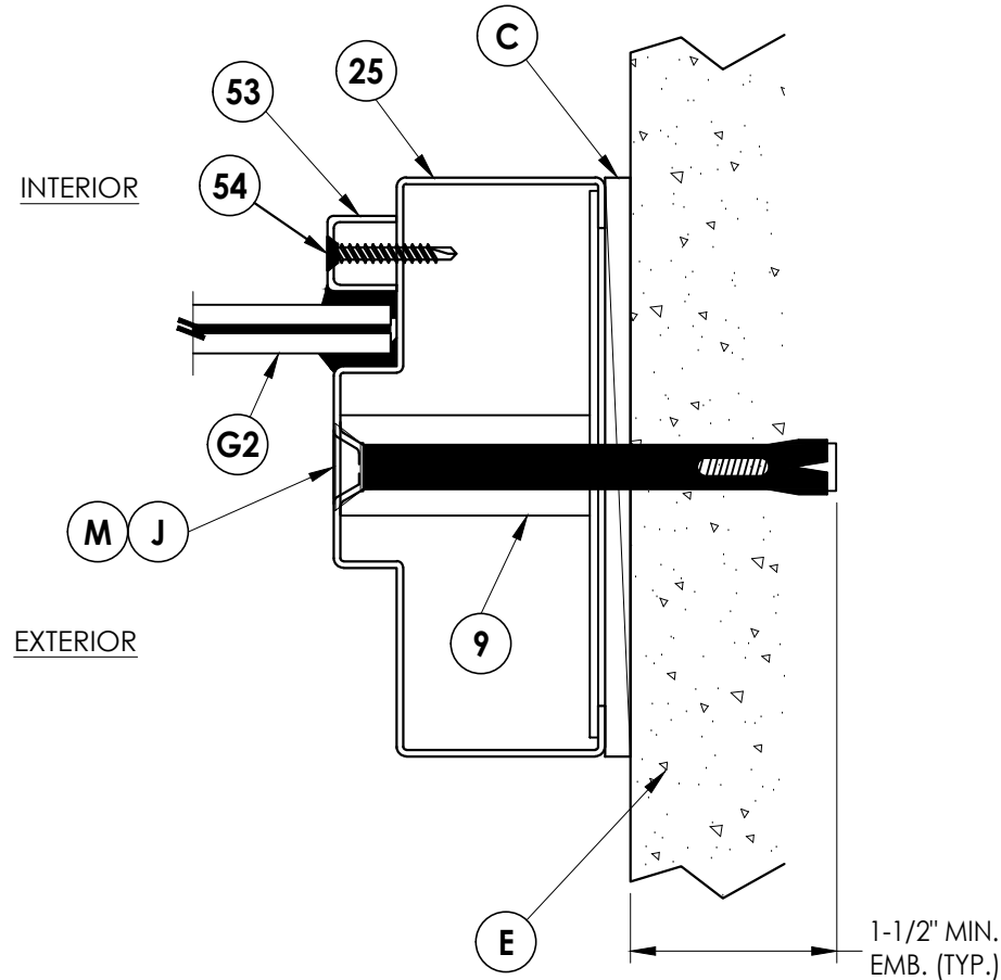
4 4 HORIZONTAL CROSS SECTION
